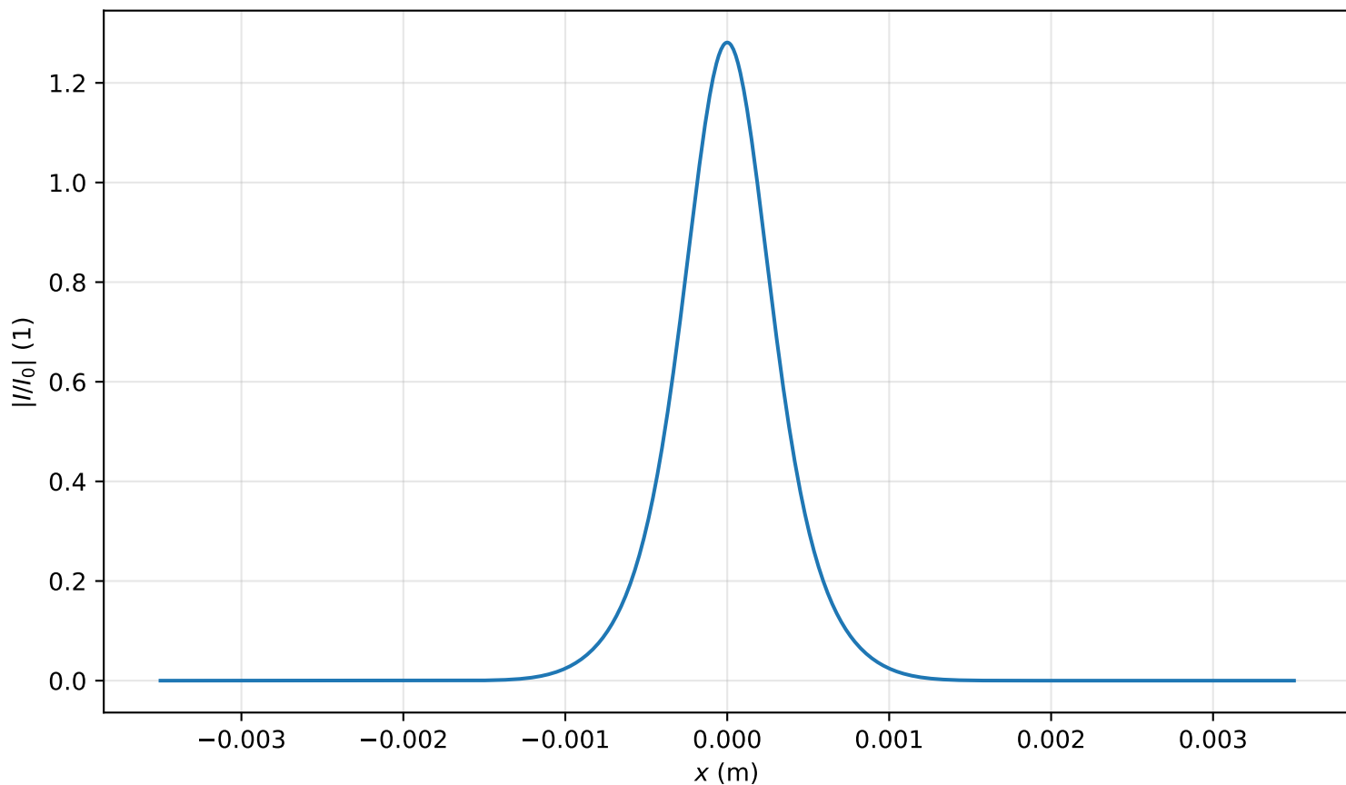
Intensity profile I(x, y = 0, z = 0.955m)/I_0 , P_{in}=0.8P_{cr} , artificial time
